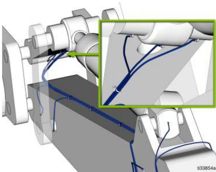
FIG. 26: Top View
