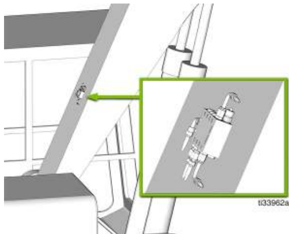
FIG. 11: Optional valve mounting if using primary valve
