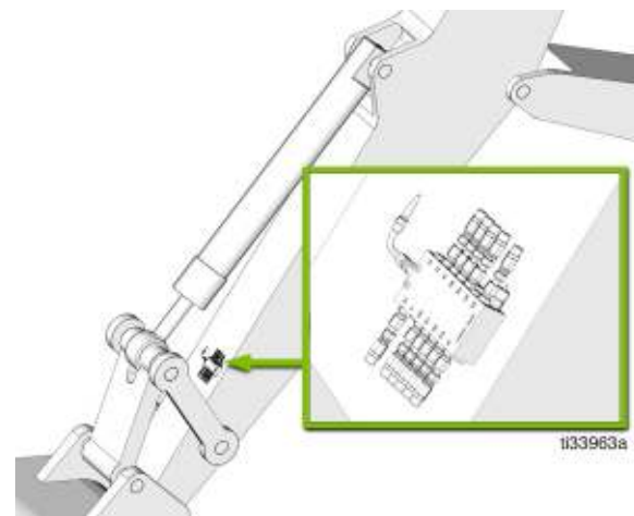
FIG. 13: Optional valve mounting
