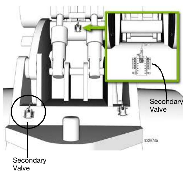
FIG. 8: Secondary Valves
