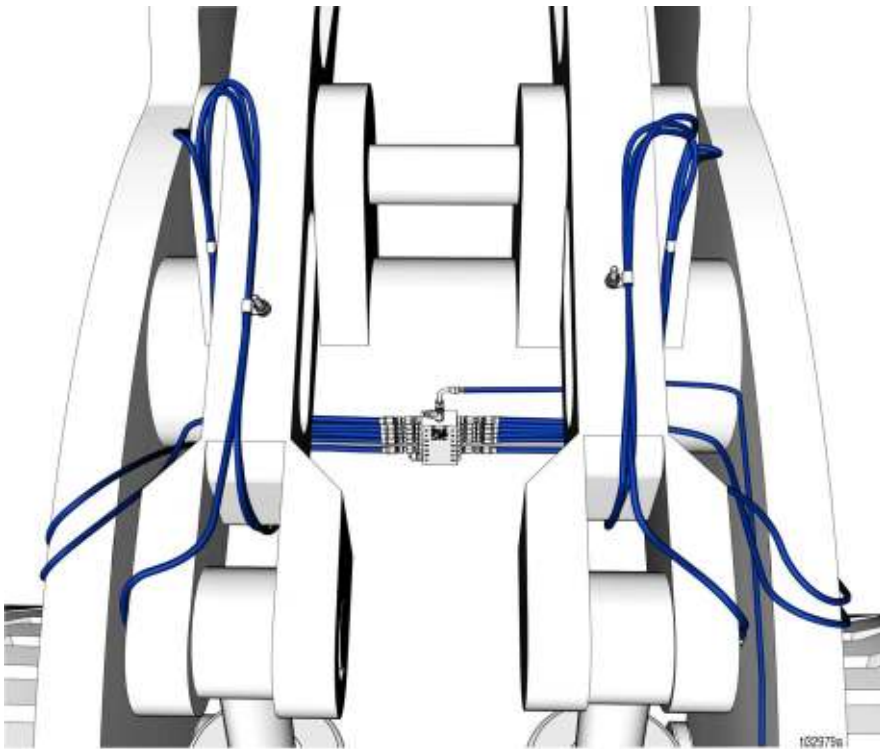
FIG. 19: Top View of Boom
